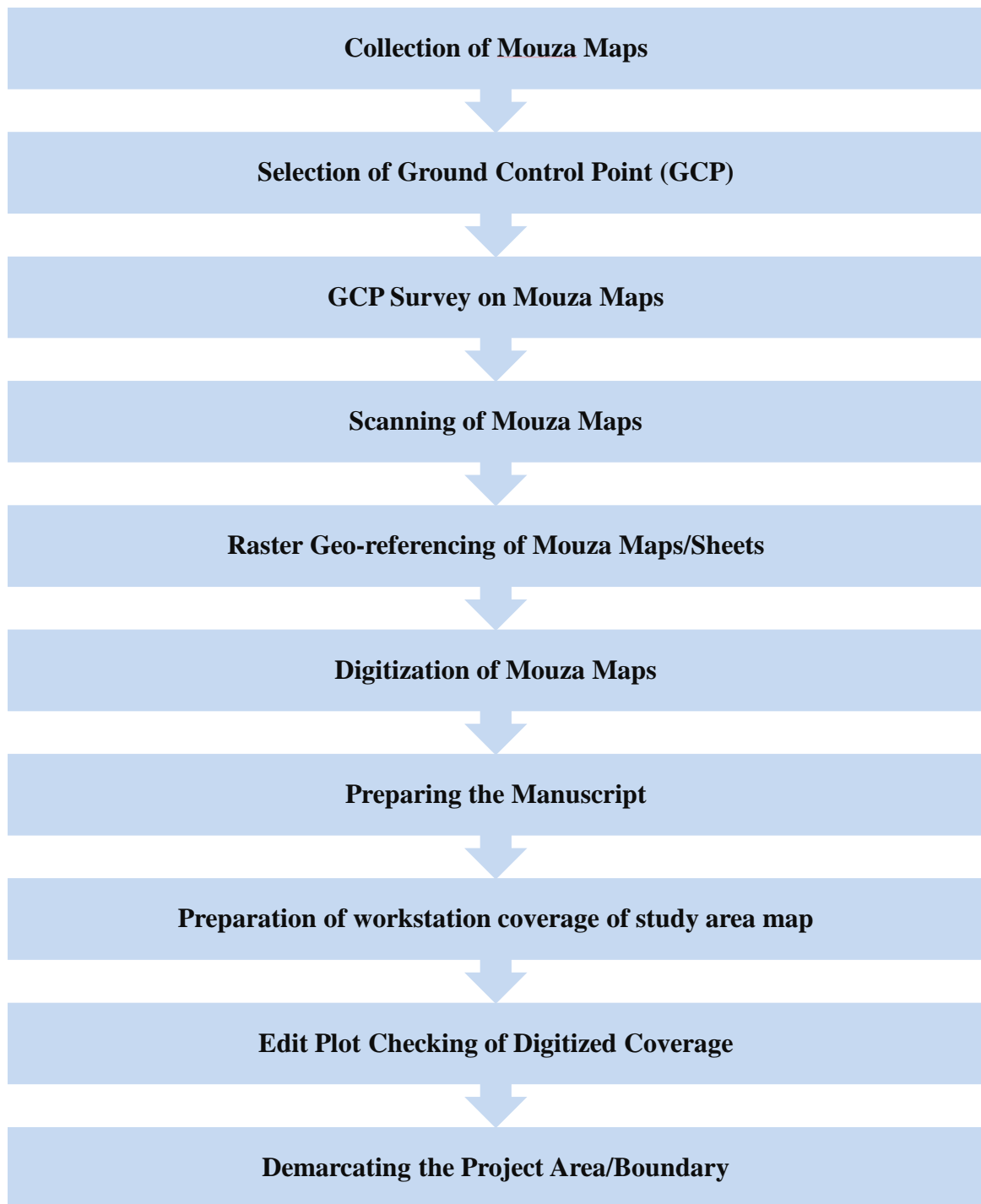
Figure 2. 1: Flow Diagram for Preparation of GIS Database using RS Mauza Map
